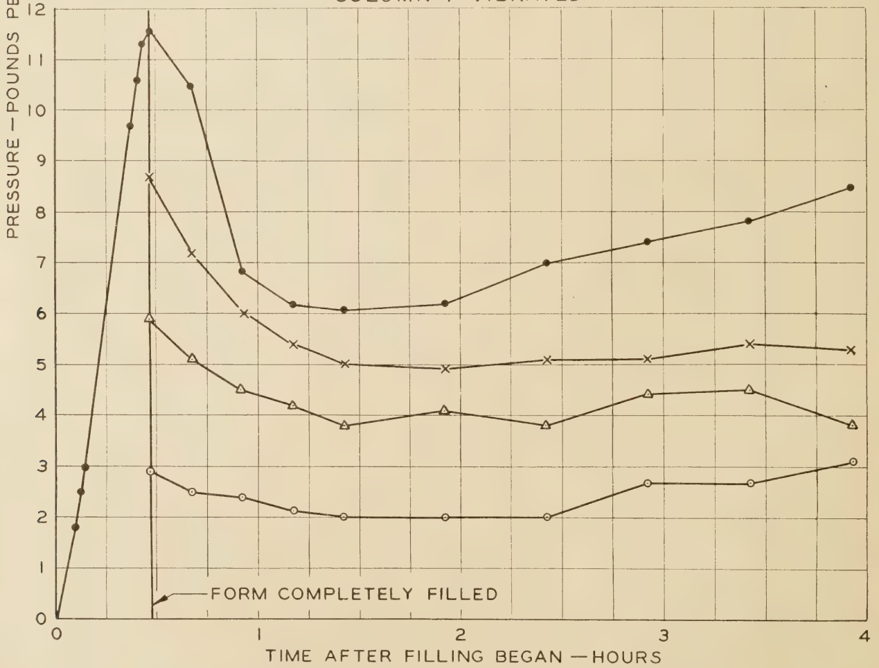
FIGURE 7.—CURVES OF PRESSURE AS A FUNCTION OF TIME FOR COLUMNS 2 AND 4
